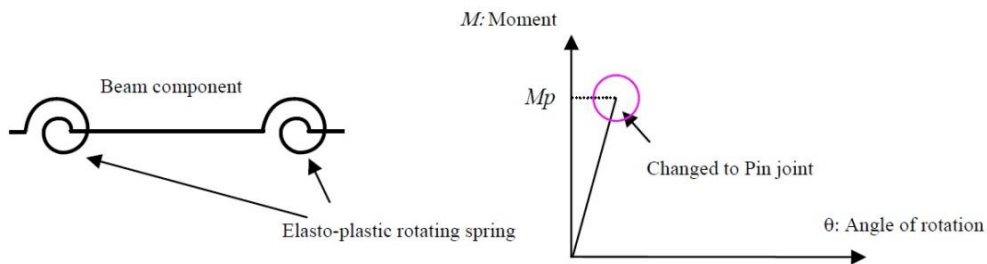
Figure 4 Schematic diagram and skeleton curve of frame spring [6]
