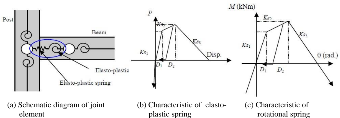
Figure 5 Outline of joint modelling [6]
