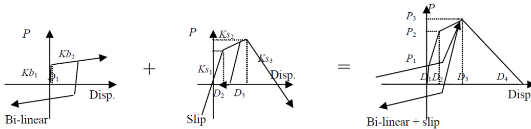
Figure 8 Hysteretic characteristics of shear wall and bracing [6]
