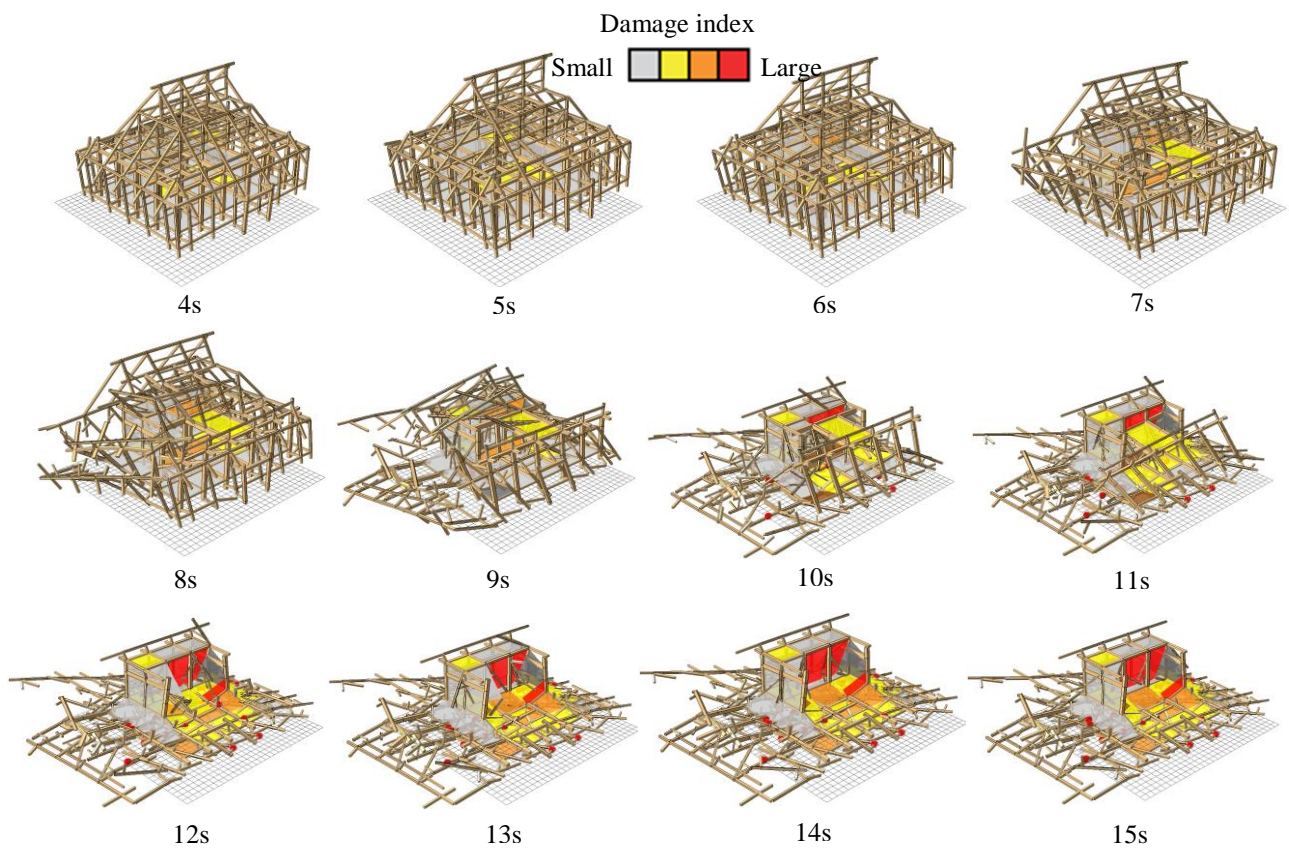
Figure 16 Seismic collapsing behaviour during the JR Takatori wave under unfixed post condition ( \mu = 0.4 )
