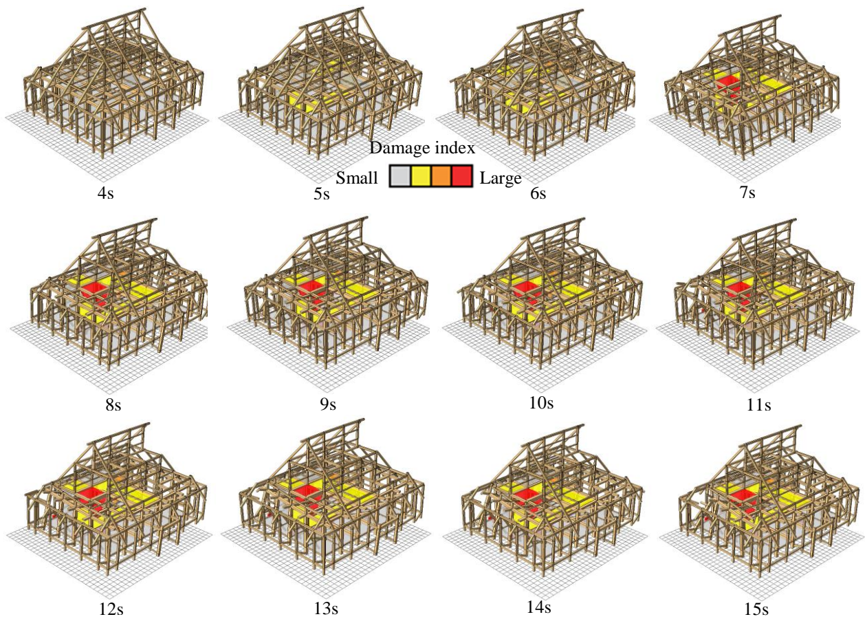
Figure 13 Seismic collapsing behaviour during the JMA Kobe wave under unfixed post condition ( \mu = 0.4 )
