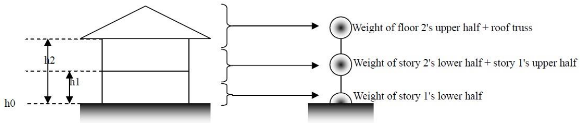
Figure 3 Weight of floor in the analytical model of wooden house [6]
