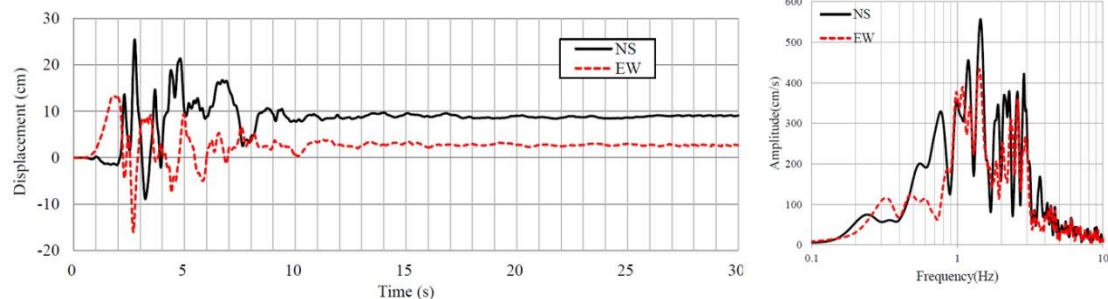
Figure 9 Displacement waves and Fourier acceleration spectra of the JMA Kobe wave
