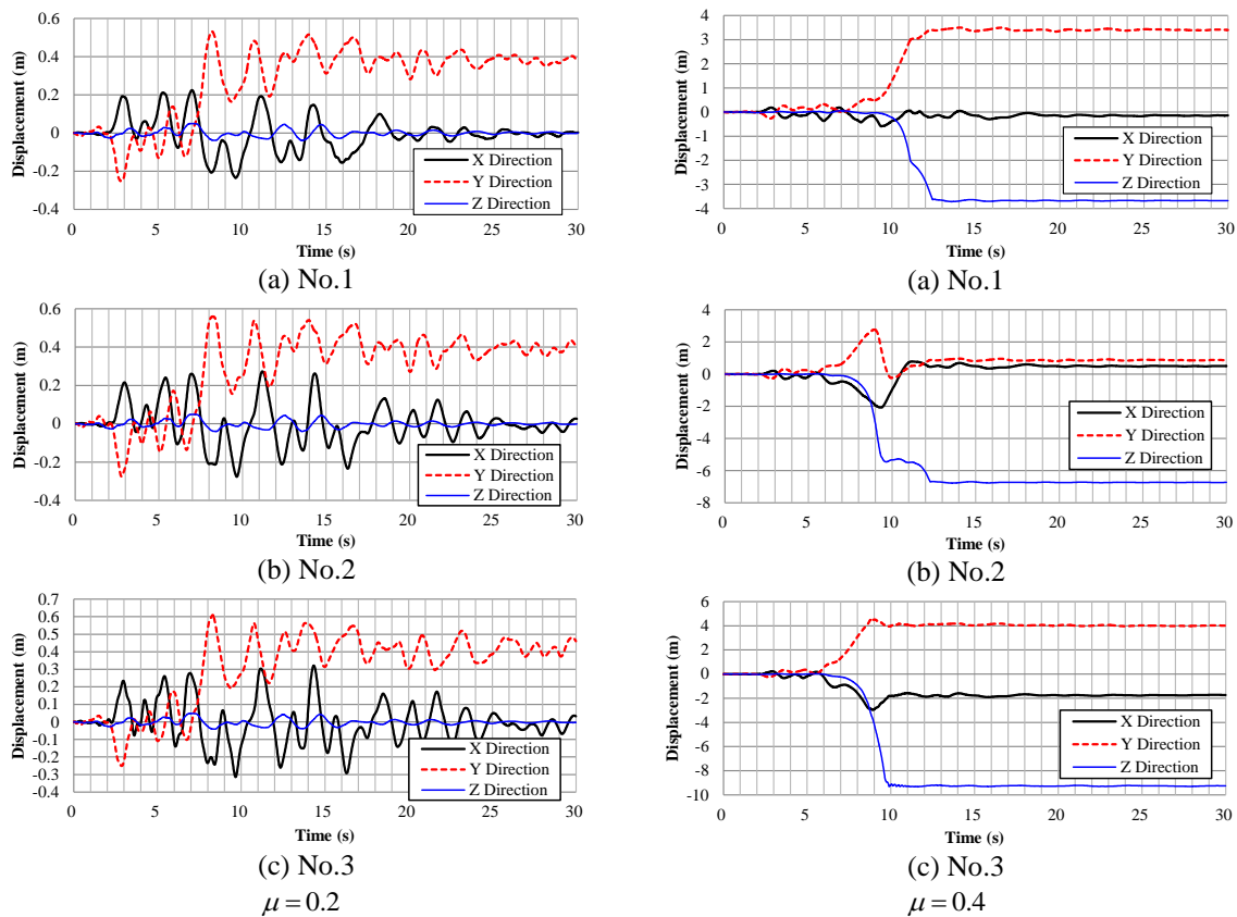
Figure 19 Displacement responses at Nos.1 to 3, the JR Takatori wave
