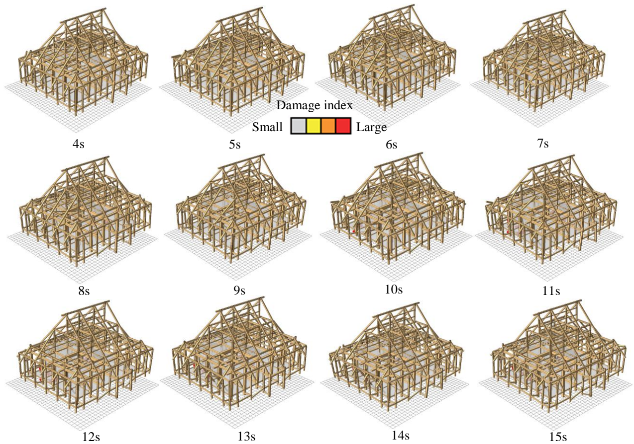
Figure 15 Seismic collapsing behaviour during the JR Takatori wave under unfixed post condition ( \mu = 0.2 )
