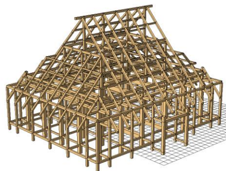
Figure 2 Collapsing wooden frame model
