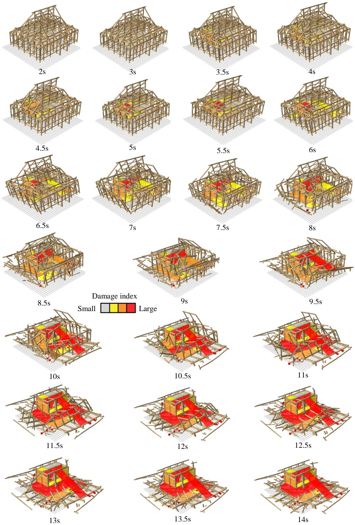
Figure 14 Seismic collapsing behaviour during the JR Takatori wave under fixed post condition
