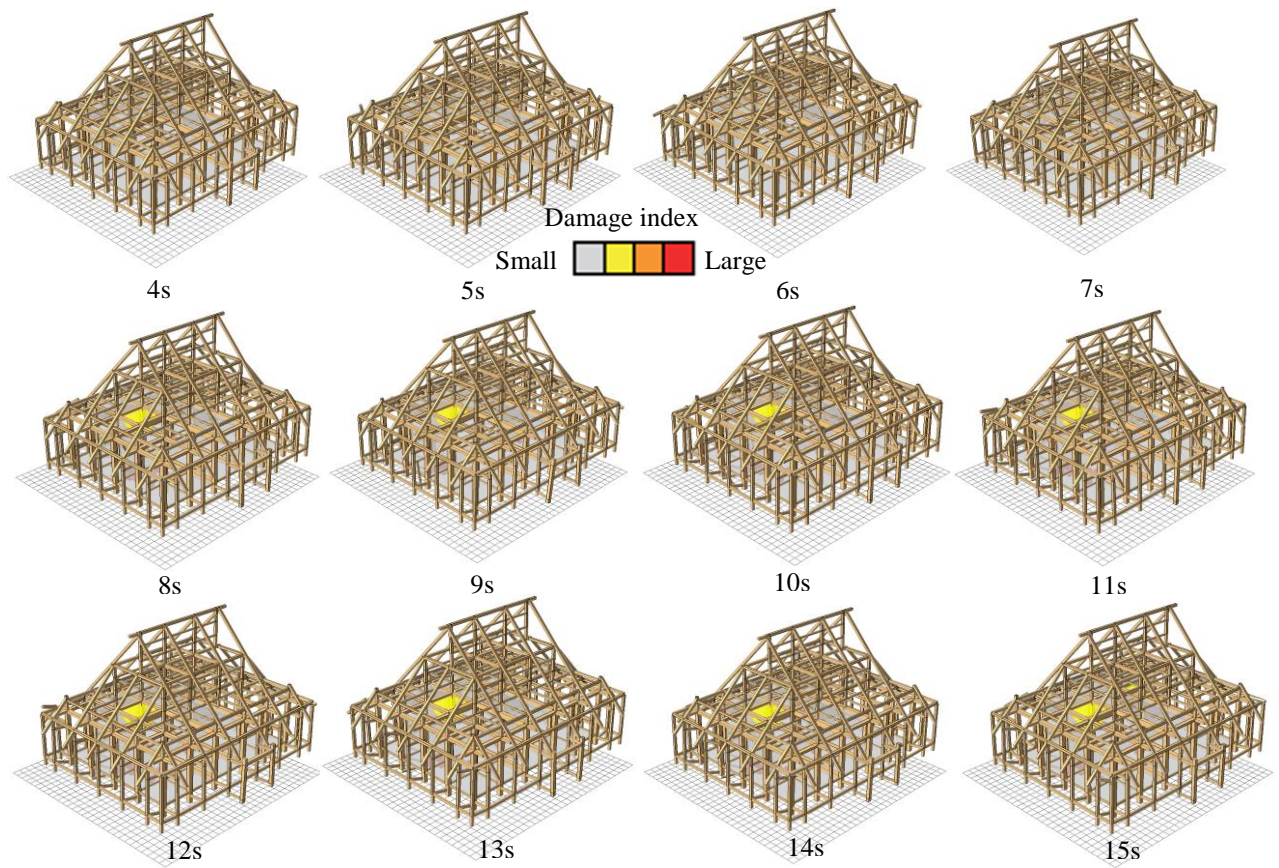
Figure 12 Seismic collapsing behaviour during the JMA Kobe wave under unfixed post condition ( \mu = 0.2 )
