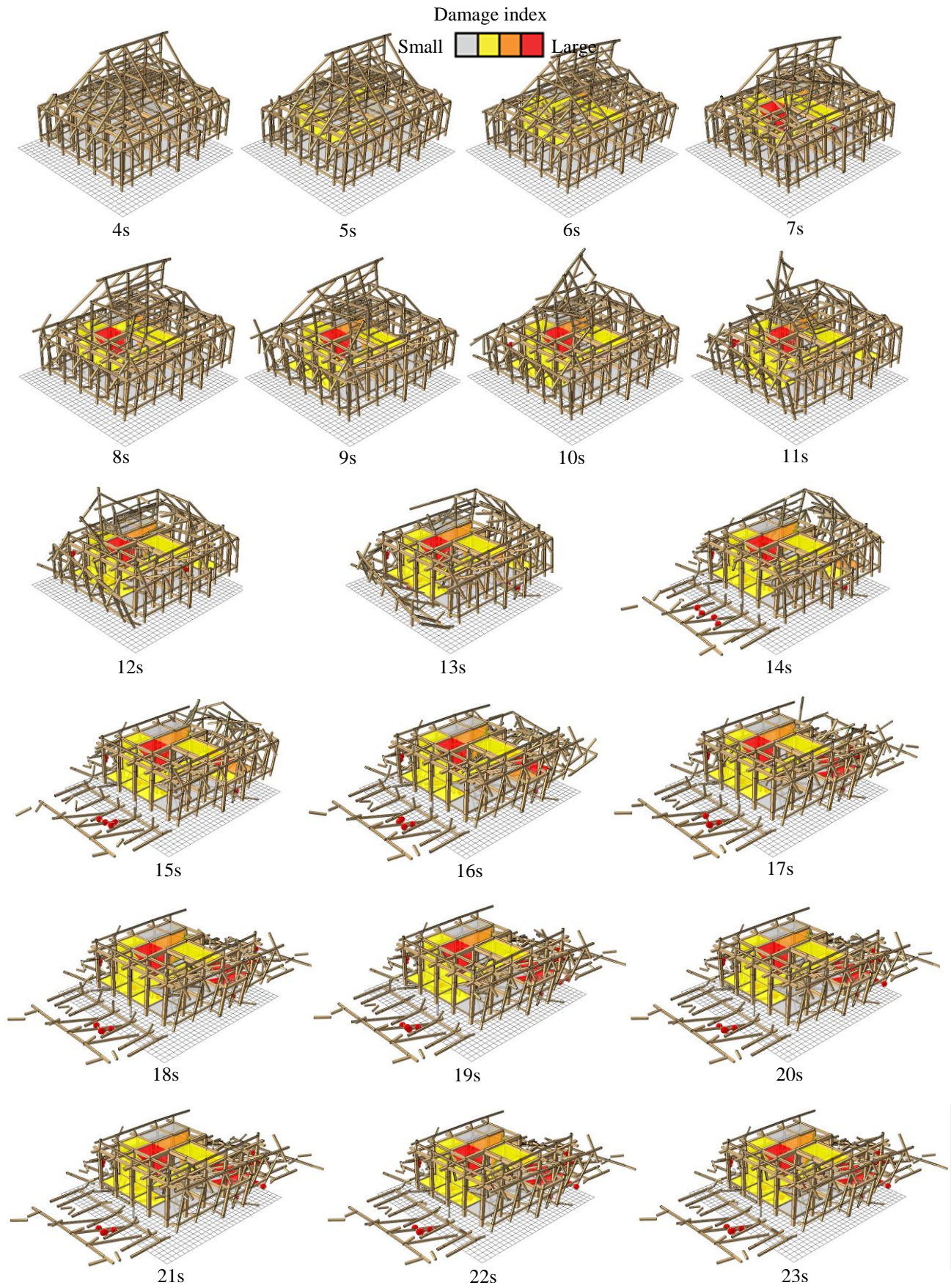
Figure 11 Seismic collapsing behaviour during the JMA Kobe wave under fixed post condition
